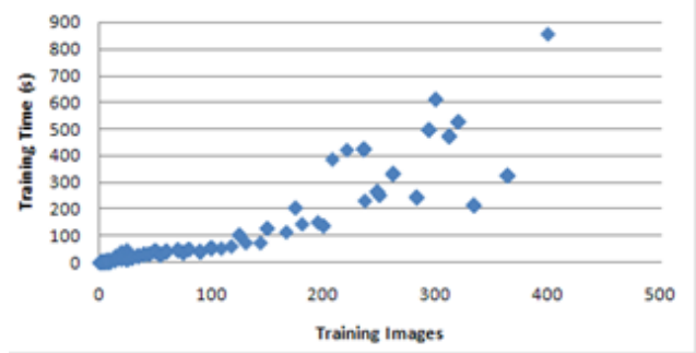
Figure 4. Time taken for training a classifier.
